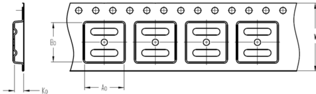
Figure 19 Specification Drawing of Reel Packaging
