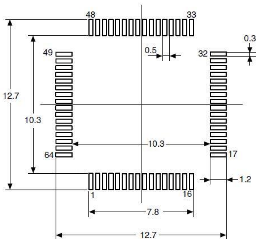
Figure 17 LQFP64-64 pins, 10×10mm recommended welding Layout
